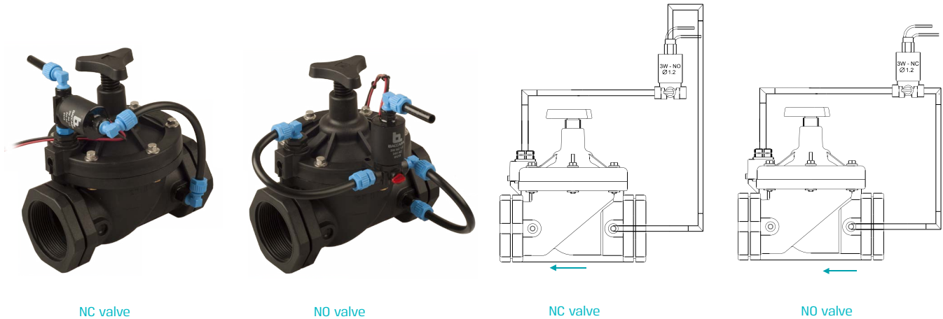
NC valve
